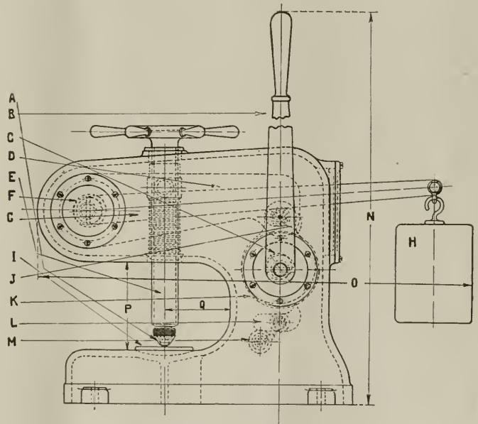
HARDNESS TESTING MACHINE
